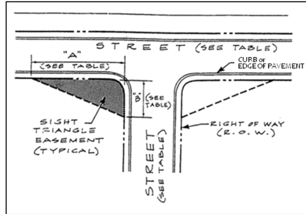
Typical Requirements By Speed Limit (Measured Along ROW Line)
